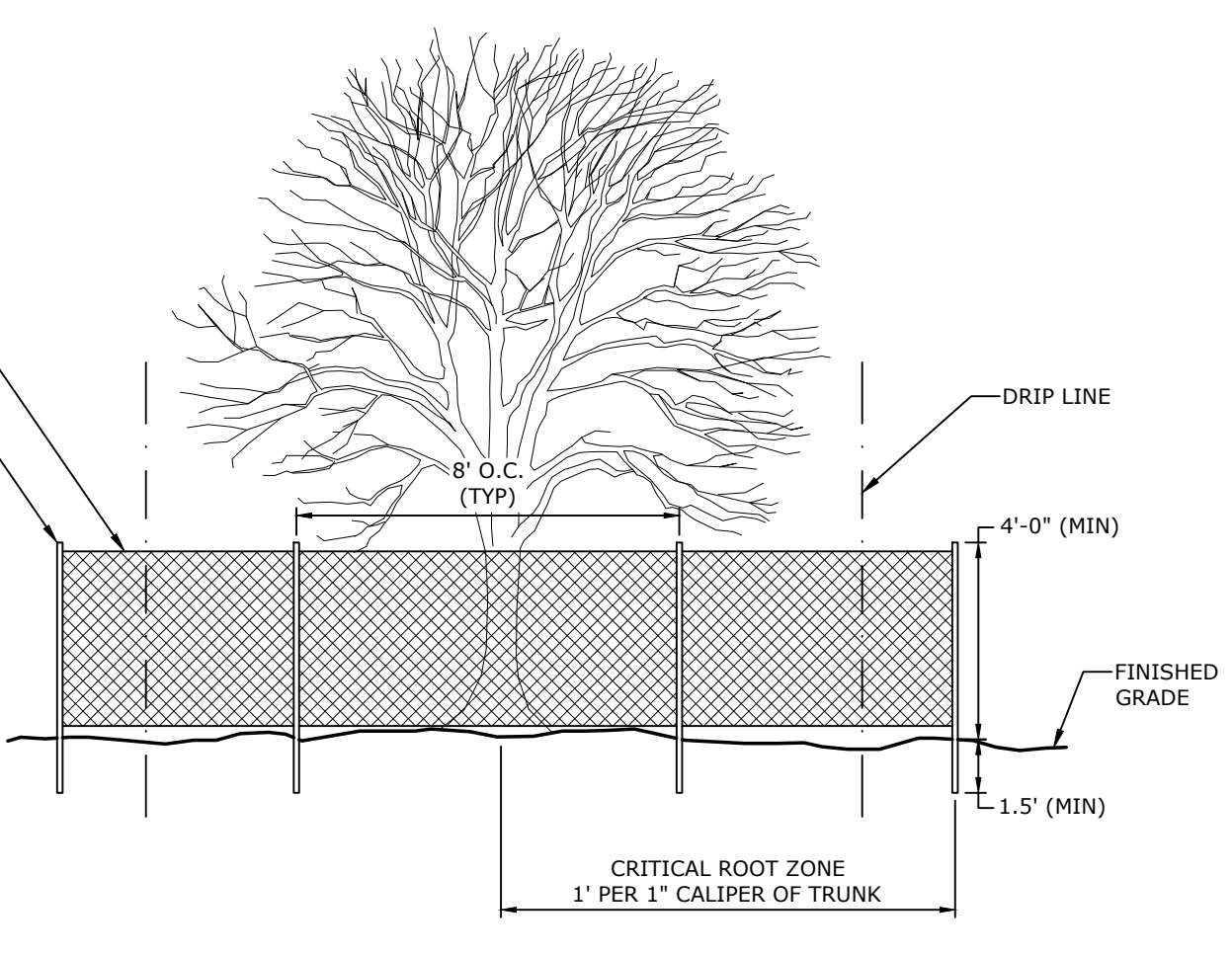
10A TREE PROTECTION FENCE NTS
